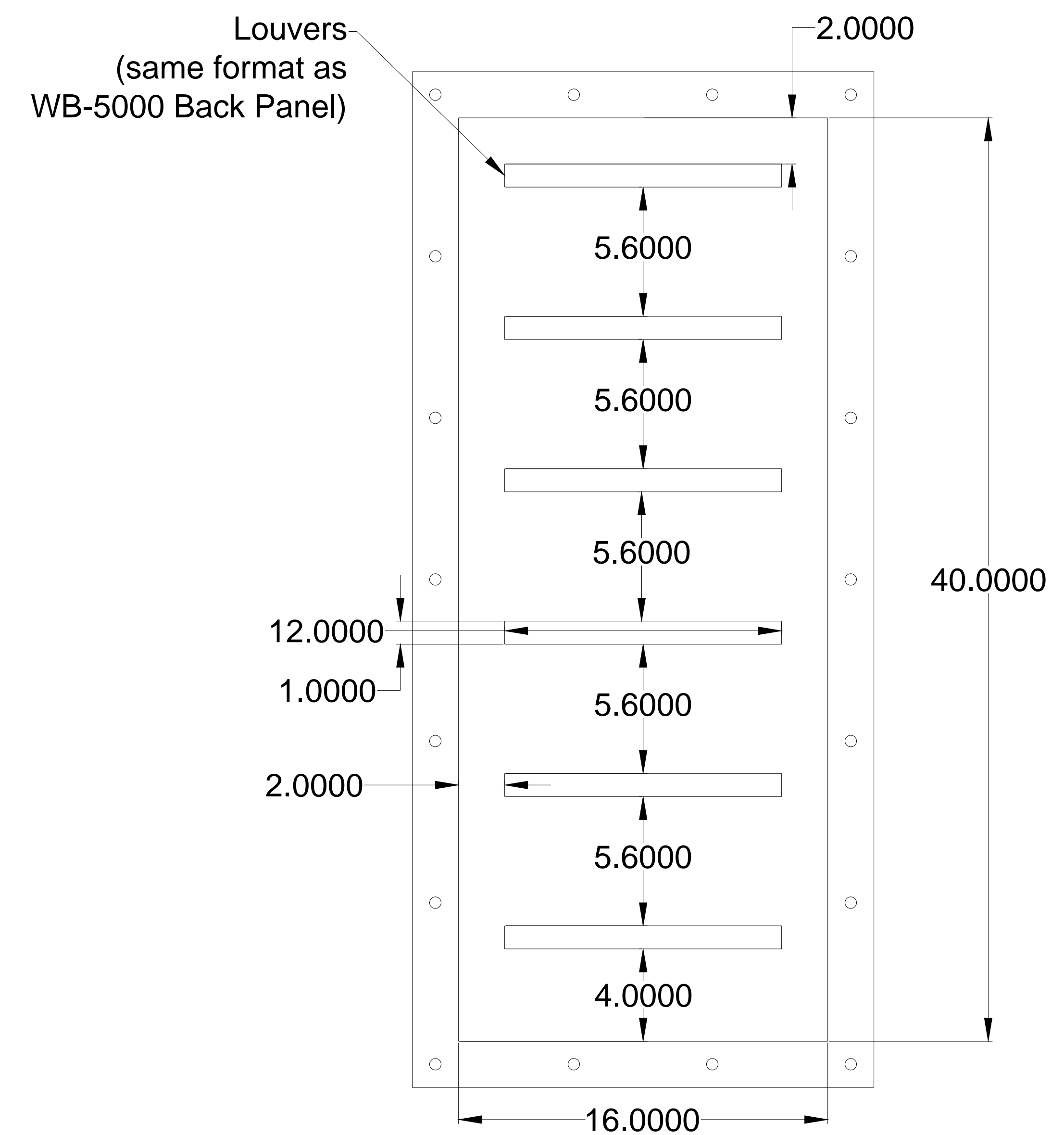
Front View
