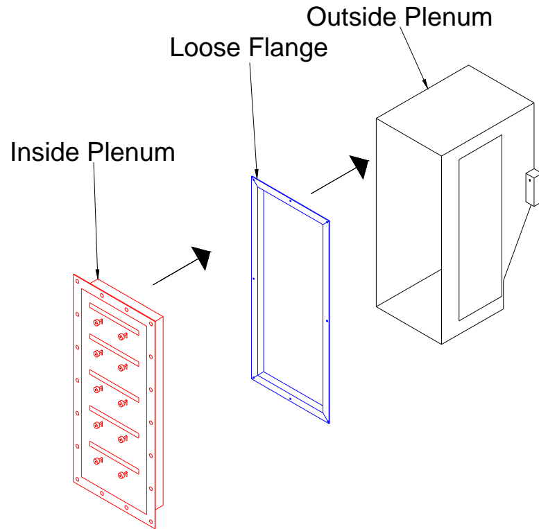
Exploded View
