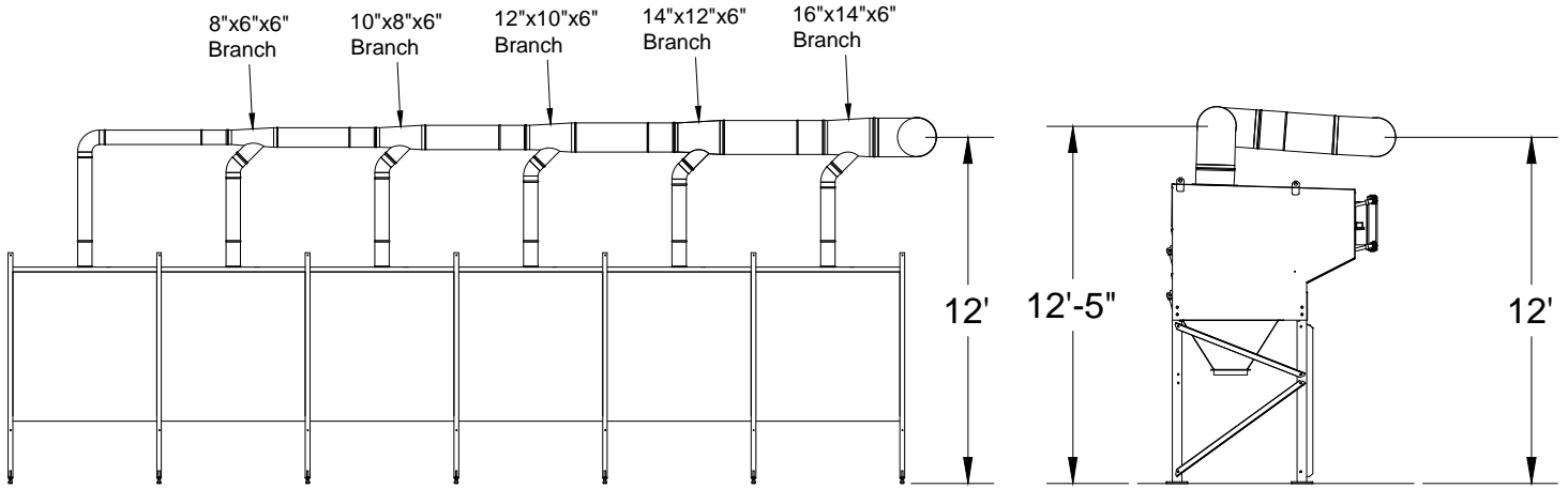
Elevation View
