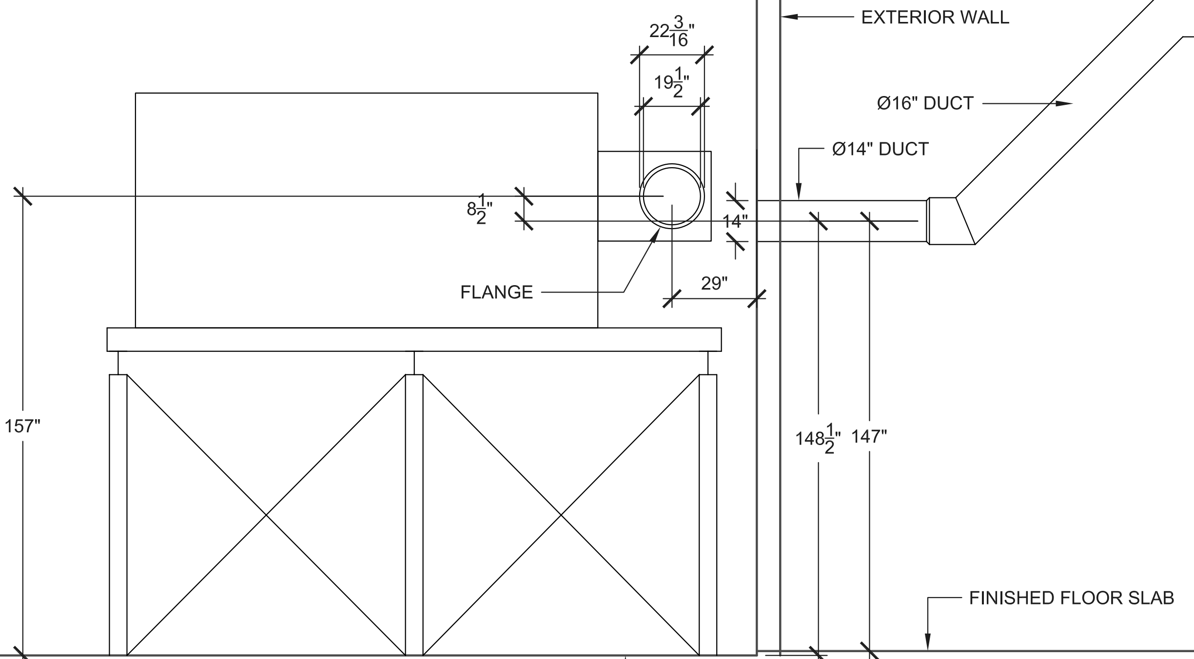
1 BUILDING SECTION @ DUST COLLECTION SCALE: 3/8" = 1' RE:
