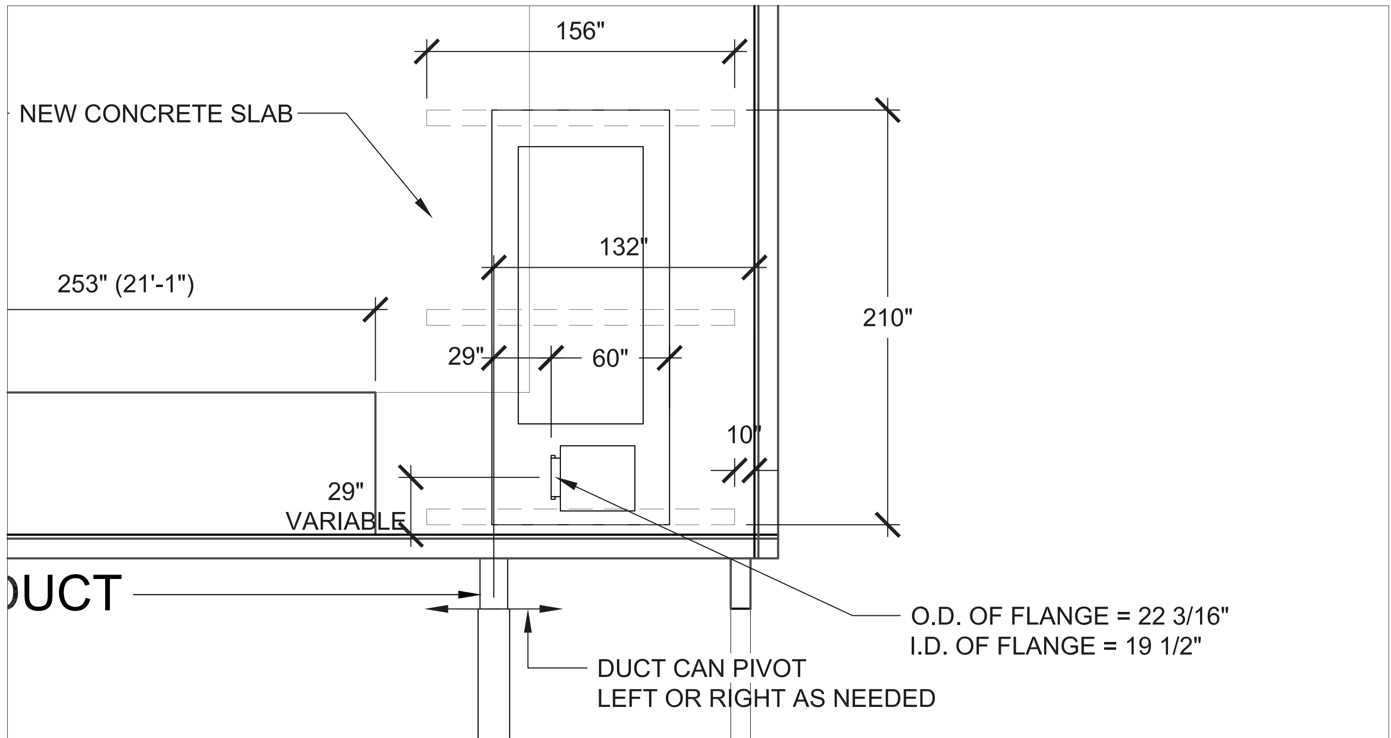
1 ENLARGED PLAN @ DUST COLLECTOR SCALE: 1/8" = 1' RE:
