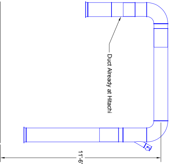
Layout A (No duct to ship)
