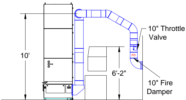
Elevation View
