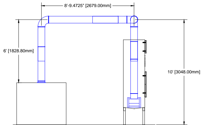
Elevation View
