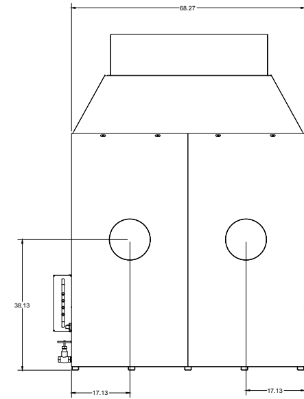
Dust Collector
