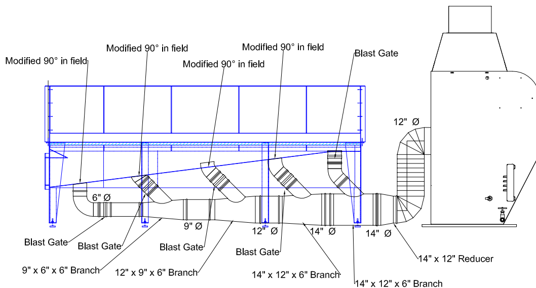
Elevation View
