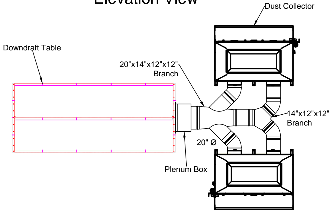
Plan View
