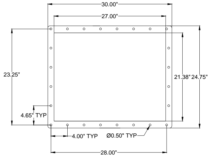
Flange View
