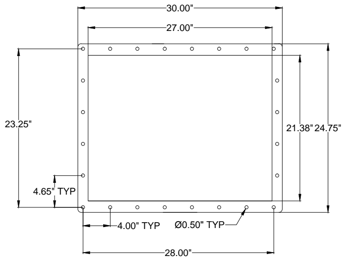
Flange View
