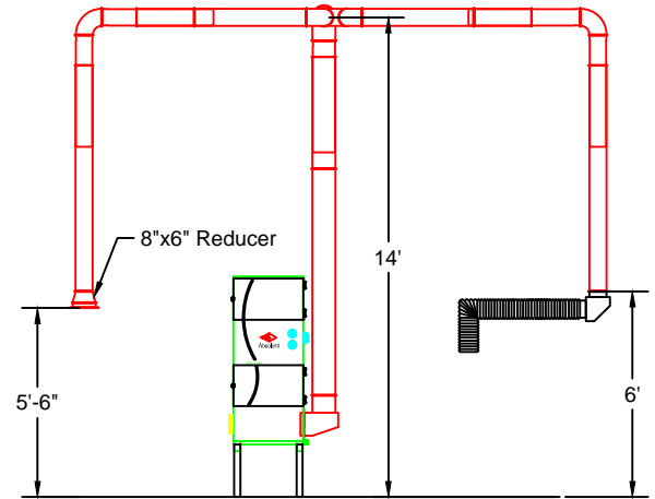
Elevation View
