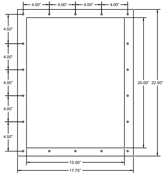
Flange View
