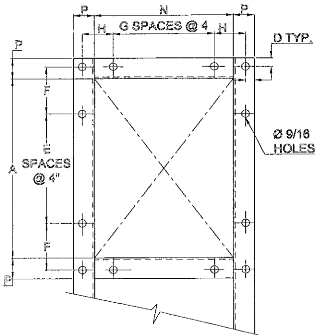
FLANGED OUTLET
