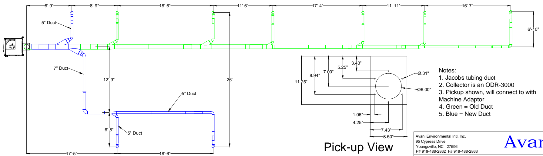
Plan View
