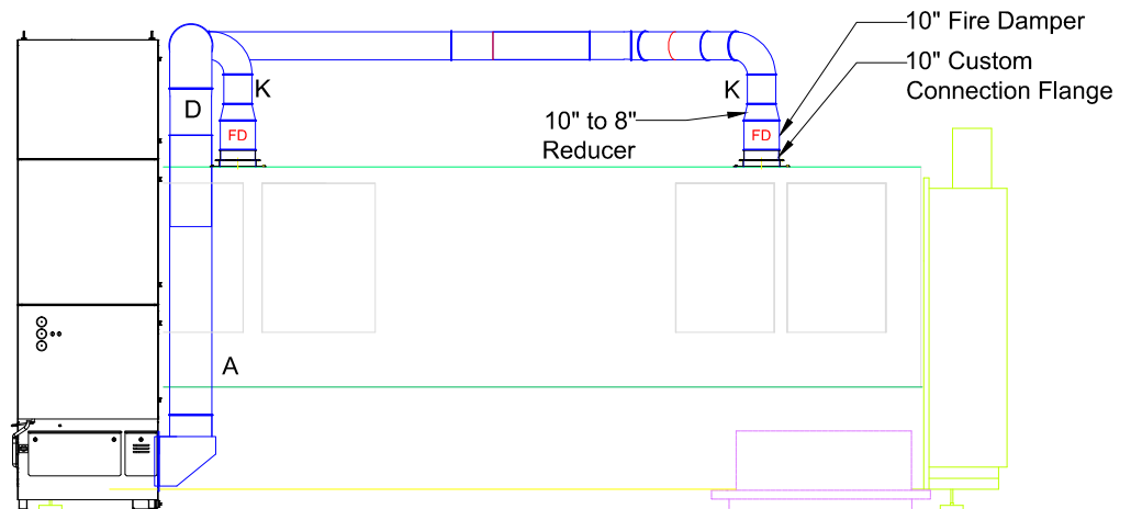
Rear View
