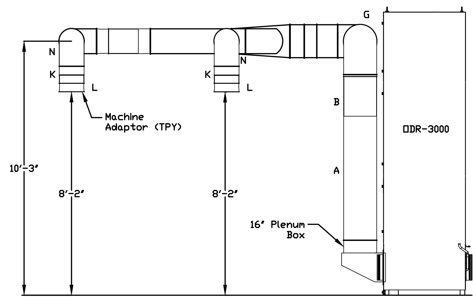
Elevation View
