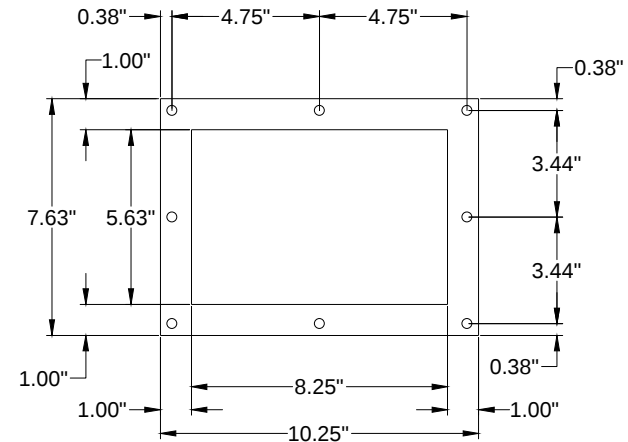
Flanged View
