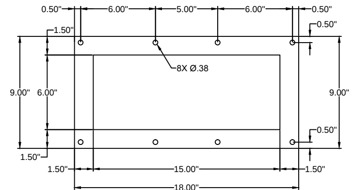
Flanged View
