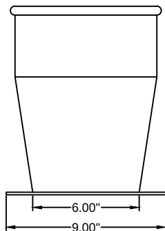
Left View
