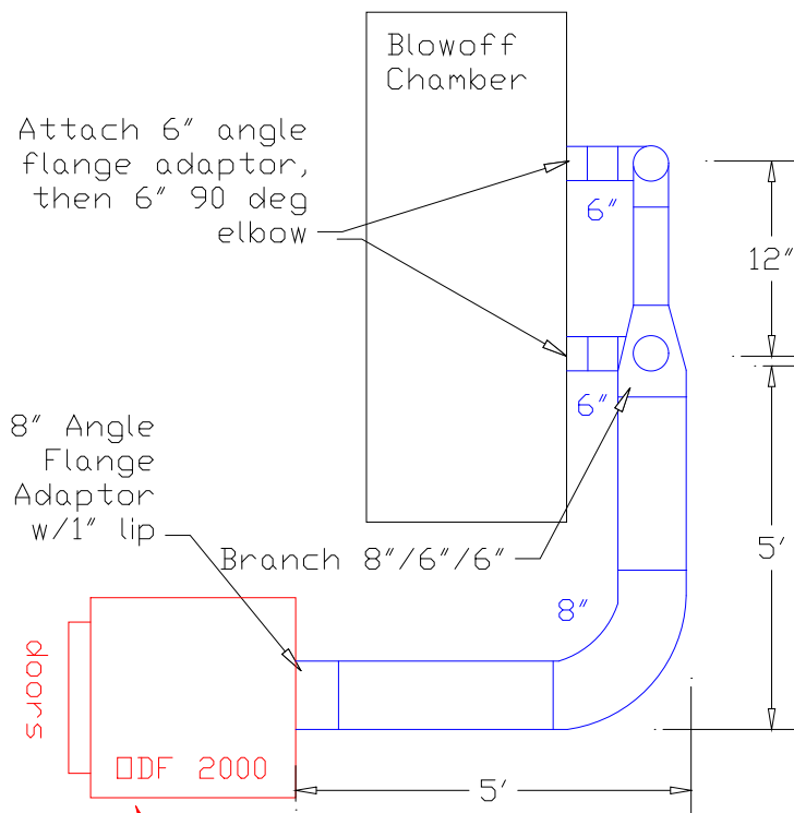
Plan View
