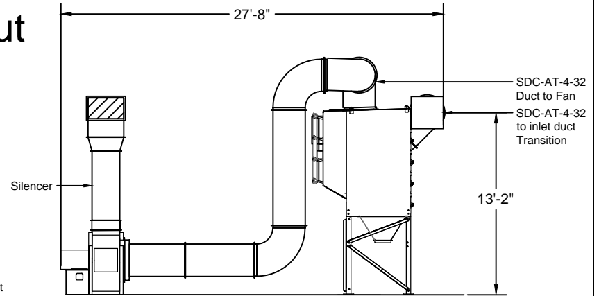
Elevation View - North Side
