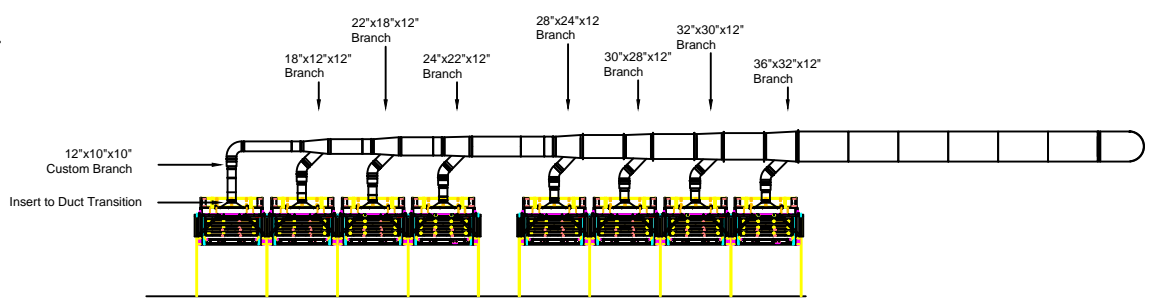
Elevation View - SDC-AT-4-48
