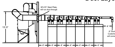
Elevation View - South Side
