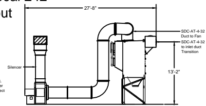
Elevation View - North Side
