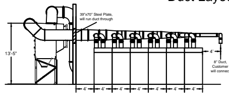
Elevation View - South Side
