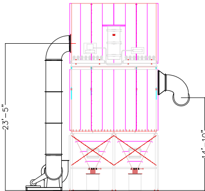
Collector Elevation View
