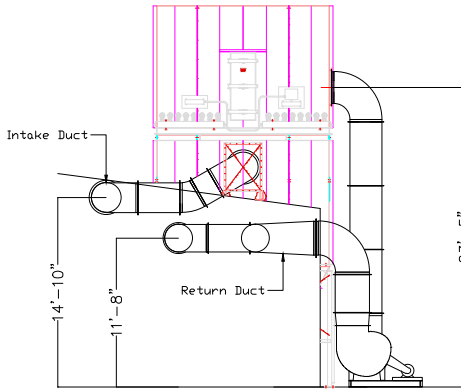
Collector Elevation View
