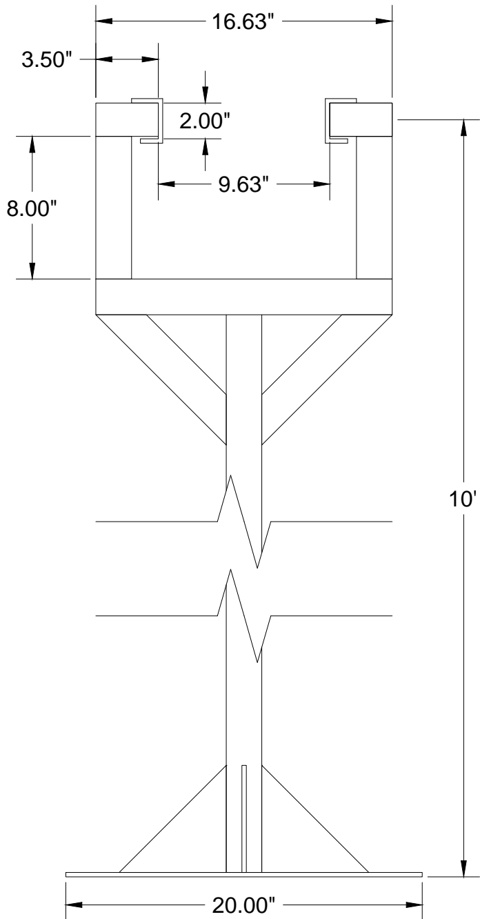
Front View
