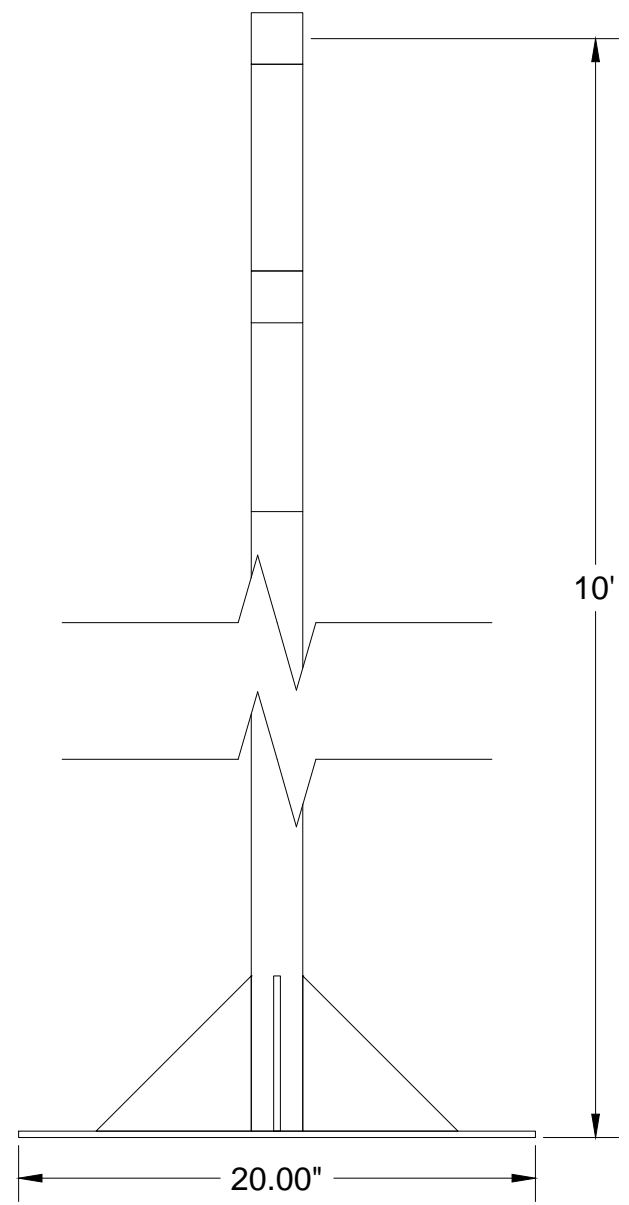
Side View
