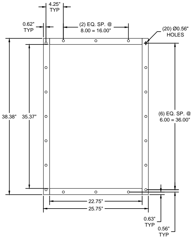
Rectangle Flange View
