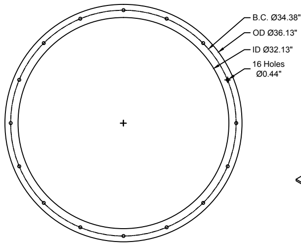
Round Flange View
