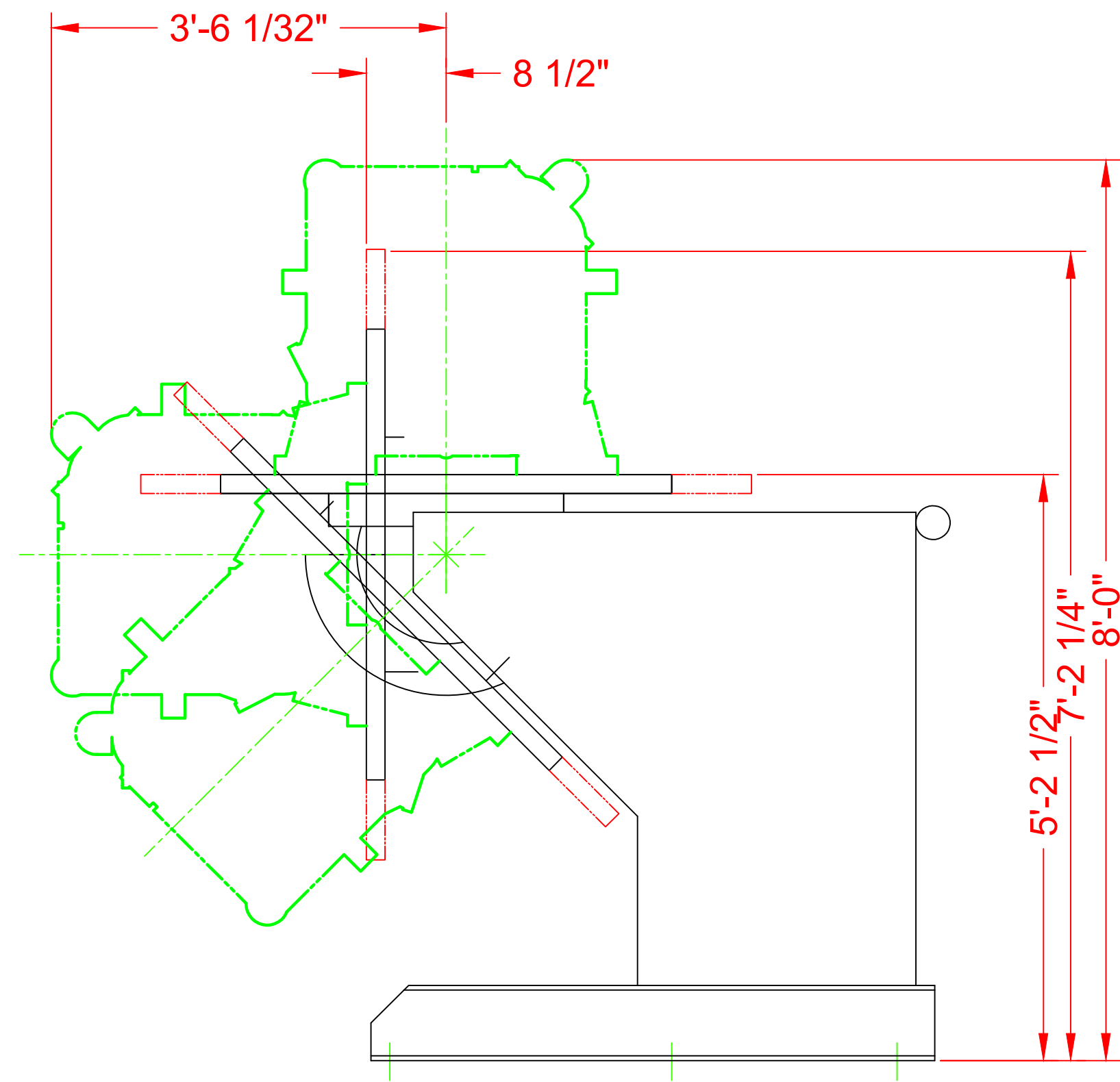
TWIN POSITIONERS QTY (2)
