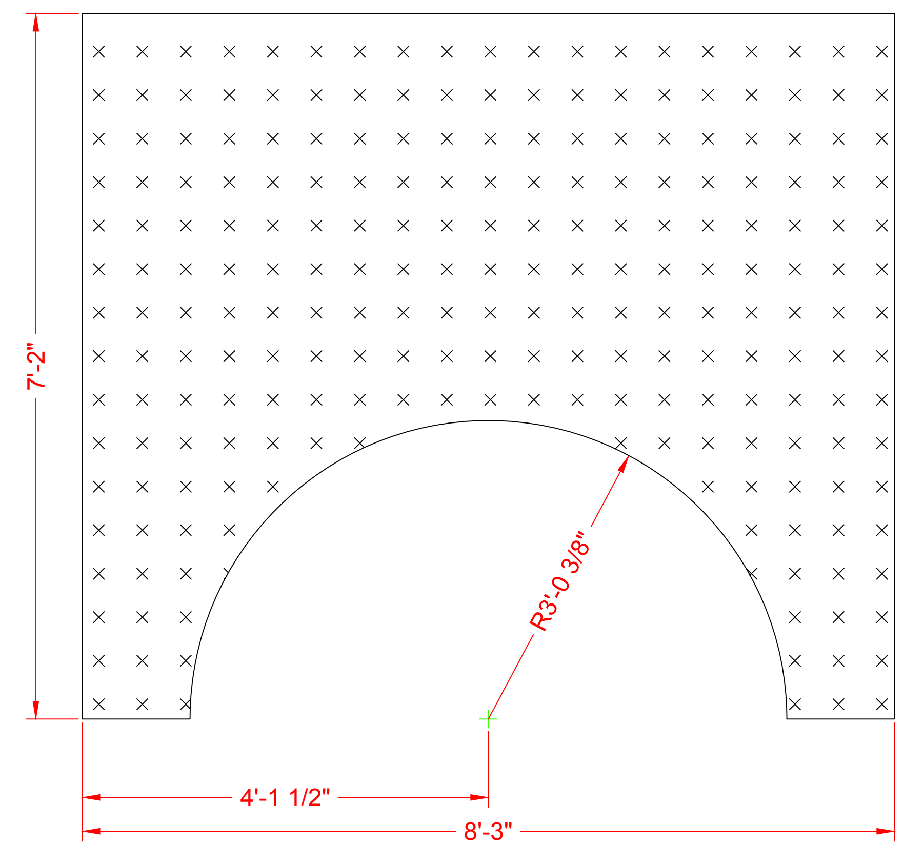
3 STEEL CHECKER PLATE 1/4 THICK X 7'-2\"/>
