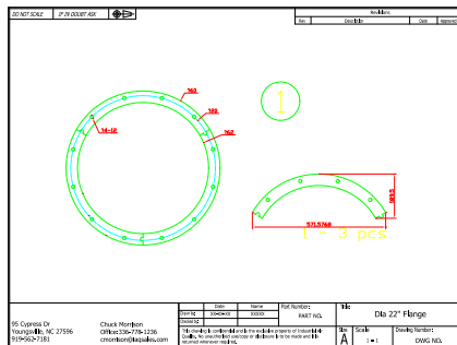
Cyclone inlet flange
