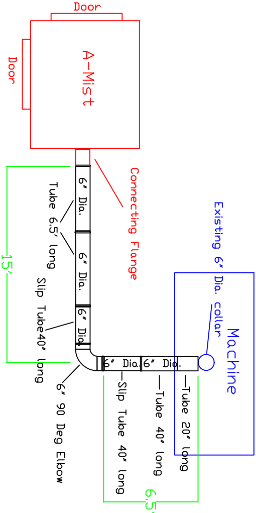
Plan View
