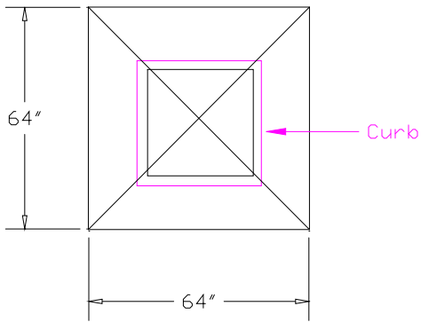
Attachment Detail
