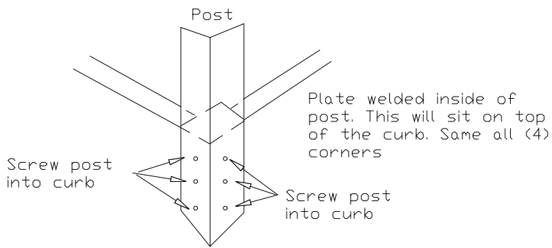
Attachment Detail
