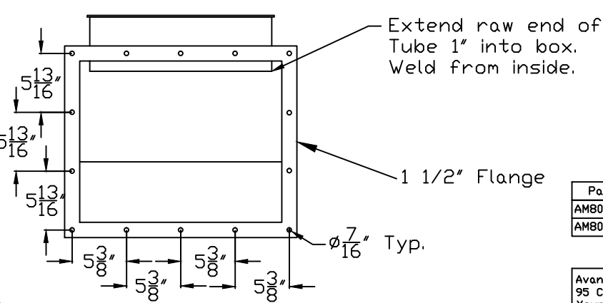
END VIEW
