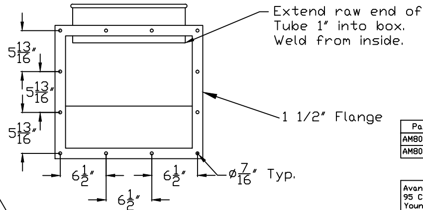
END VIEW
