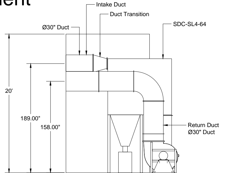
Elevation Side View
