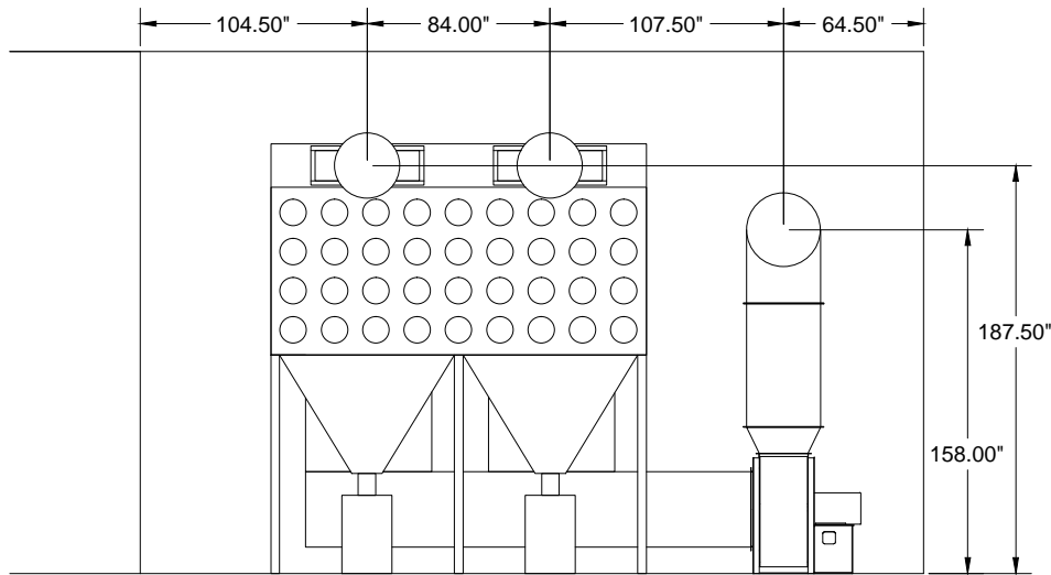
Elevation Back View
