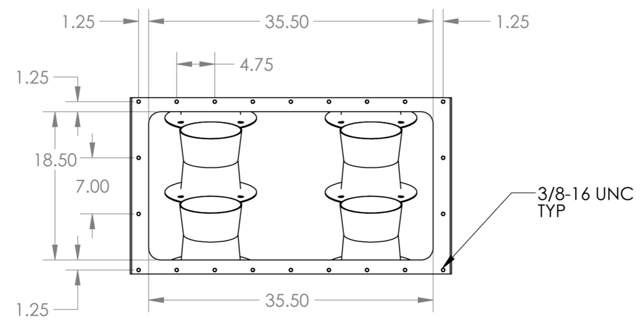
SECTION C-C
